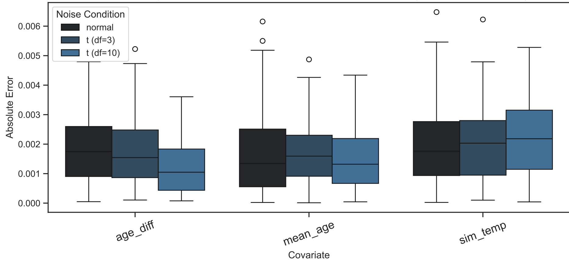
Absolute Error by Covariate Coefficient, Innovation Distribution (No Interaction Term): ER
