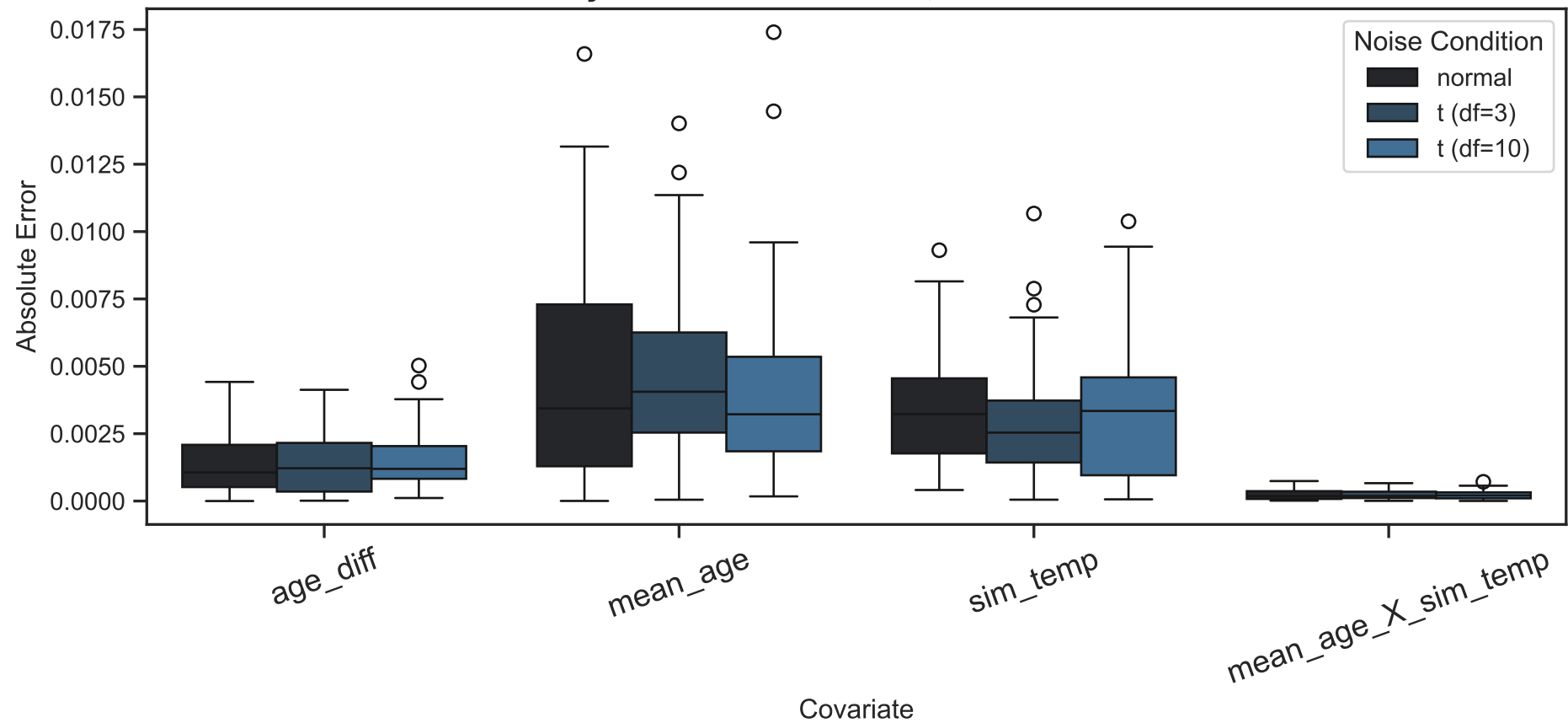
Absolute Error by Covariate Coefficient, Innovation Distribution: RDP
