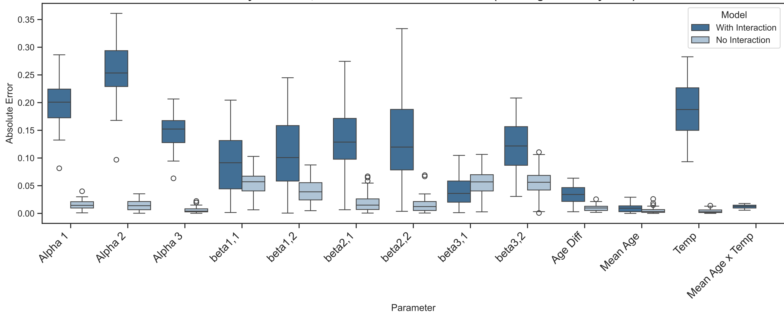
Absolute Error by Parameter, With vs Without Interaction Term (Rewiring Probability = 0.2): RDP
