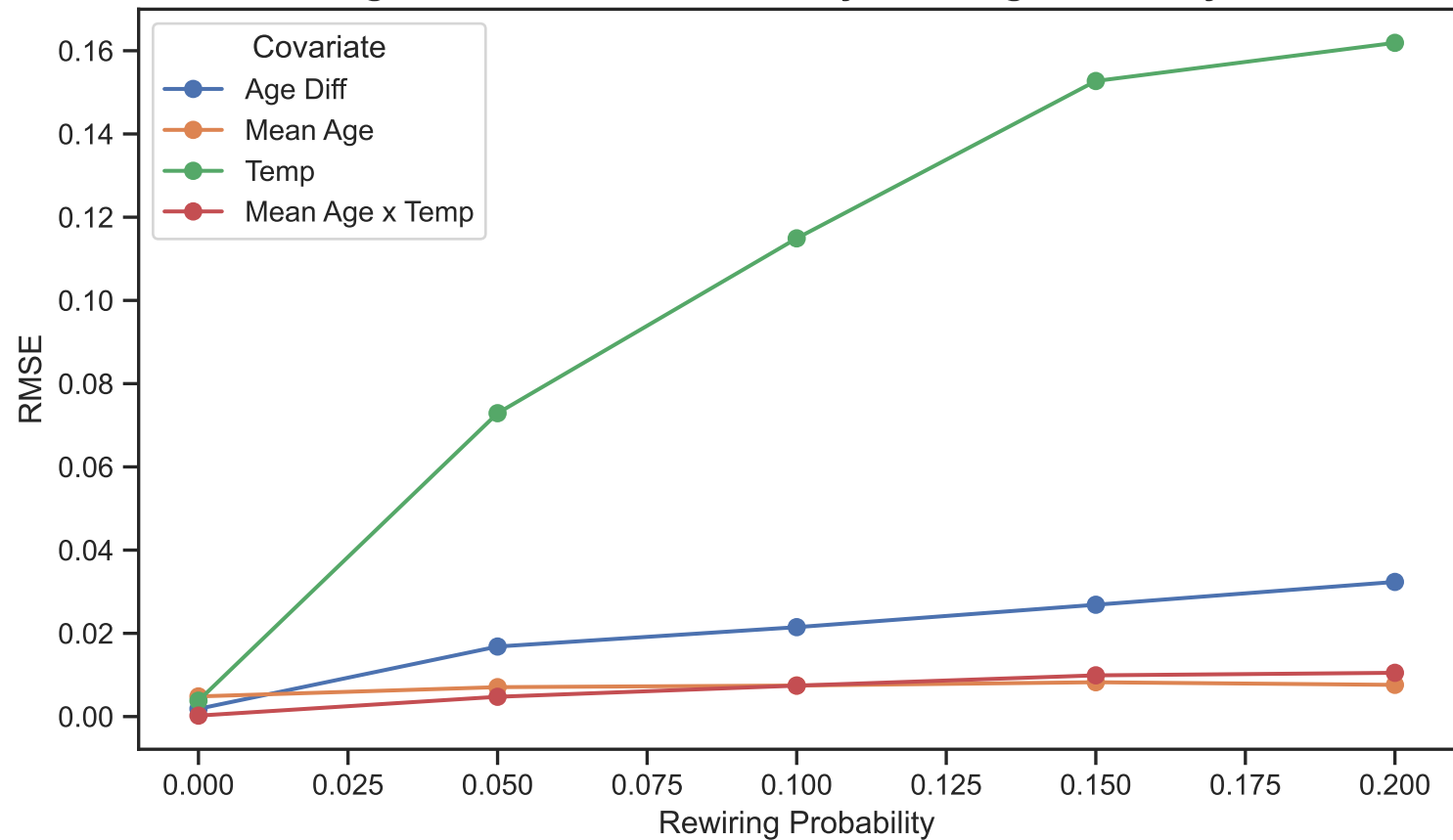
Exogenous Coefficient RMSE by Rewiring Probability: ER
