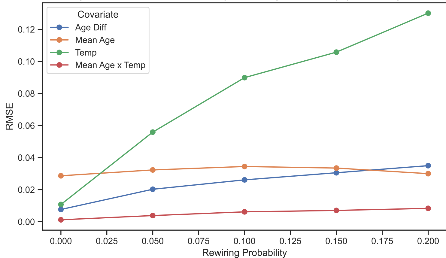
Exogenous Coefficient RMSE by Rewiring Probability (13 nodes): SBM
