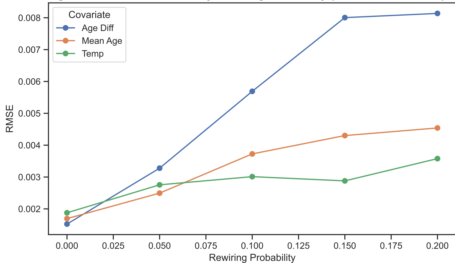
Exogenous Coefficient RMSE by Rewiring Probability (No Interaction Term): ER
