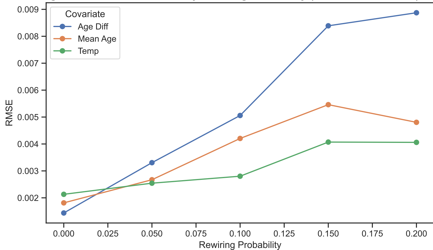
Exogenous Coefficient RMSE by Rewiring Probability (No Interaction Term): SBM
