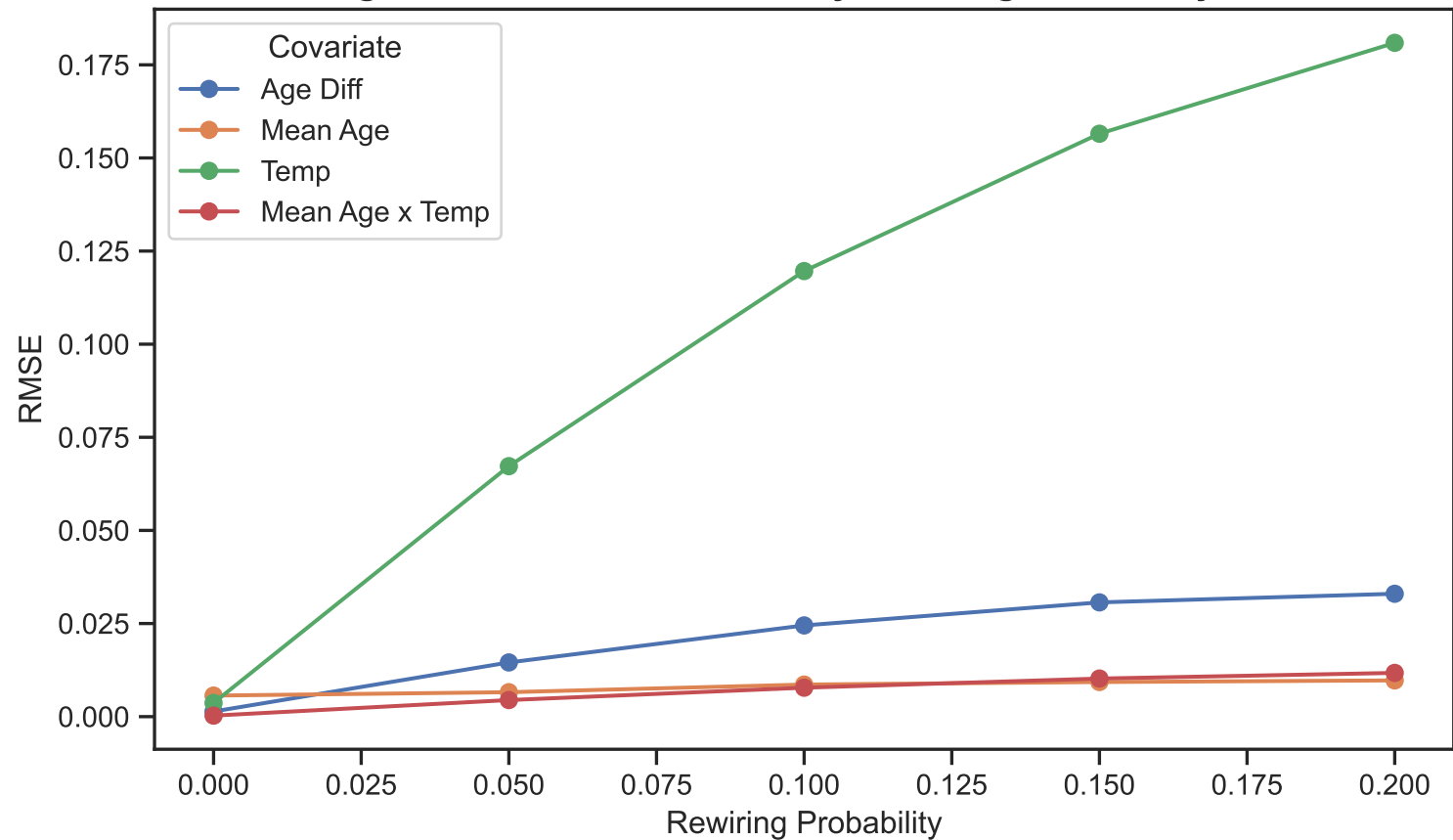
Exogenous Coefficient RMSE by Rewiring Probability: SBM
