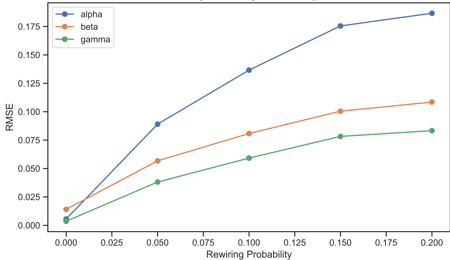
RMSE by Rewiring Probability: ER
