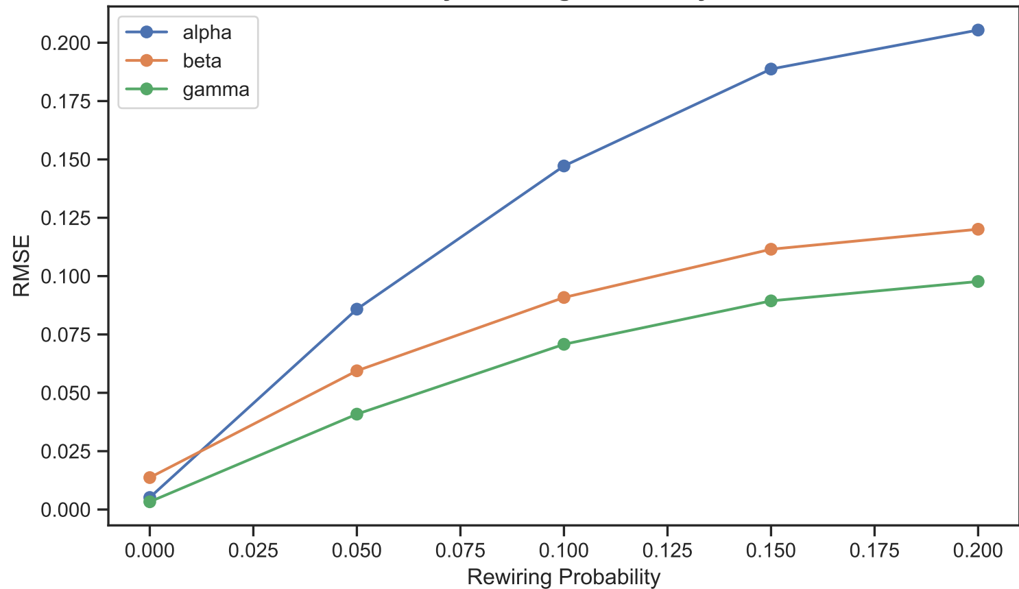
RMSE by Rewiring Probability: RDP
