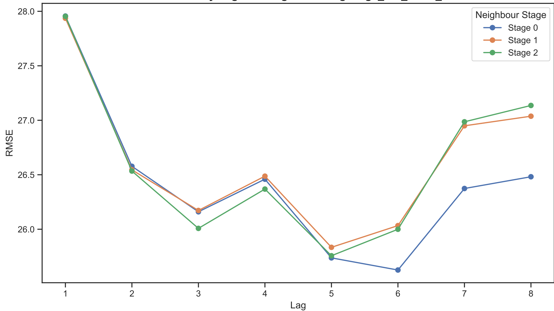
Mean RMSE by Lag and Neighbour Stage: age_diff_same_sex
