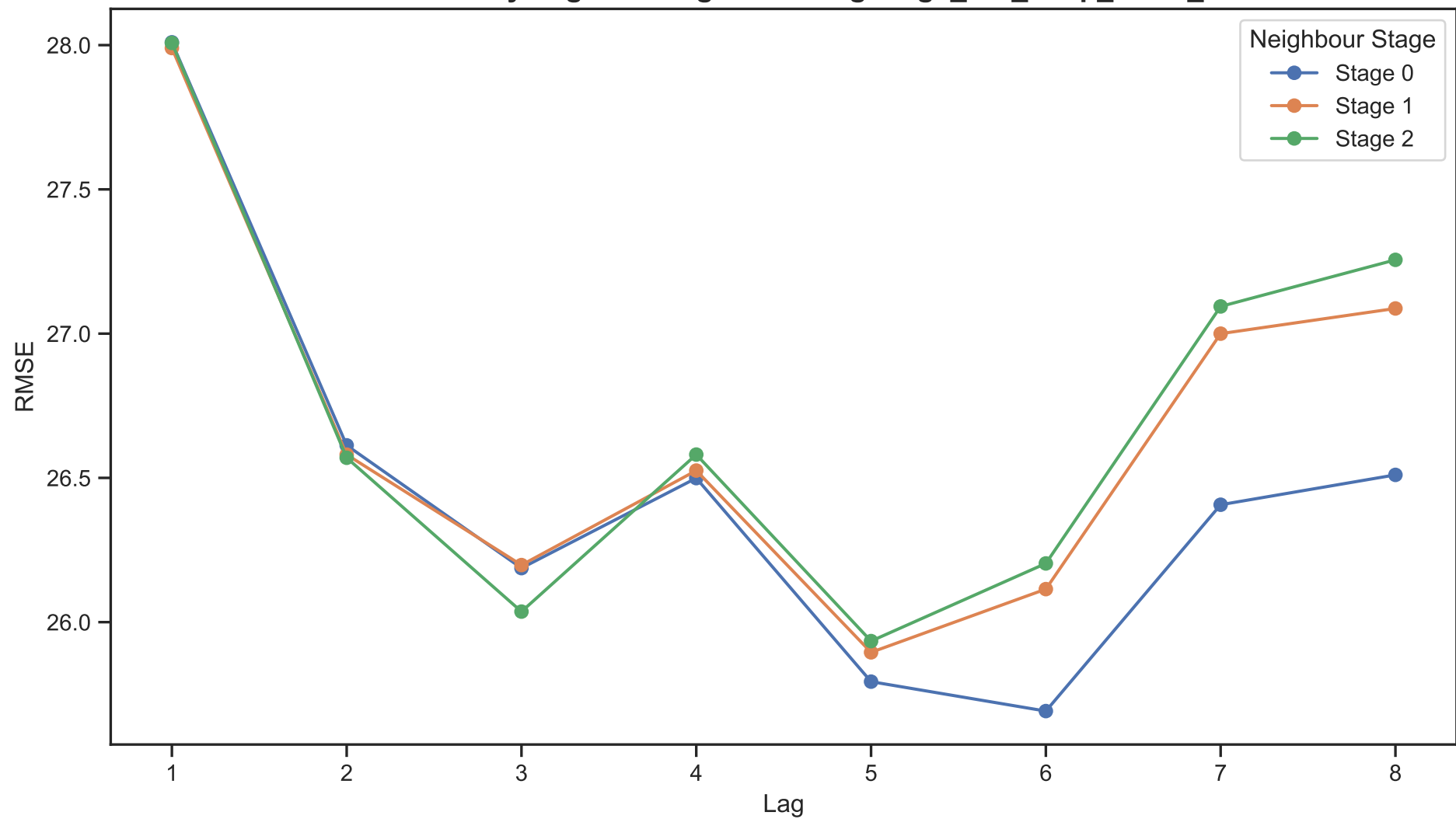
Mean RMSE by Lag and Neighbour Stage: age_diff_temp_same_sex
