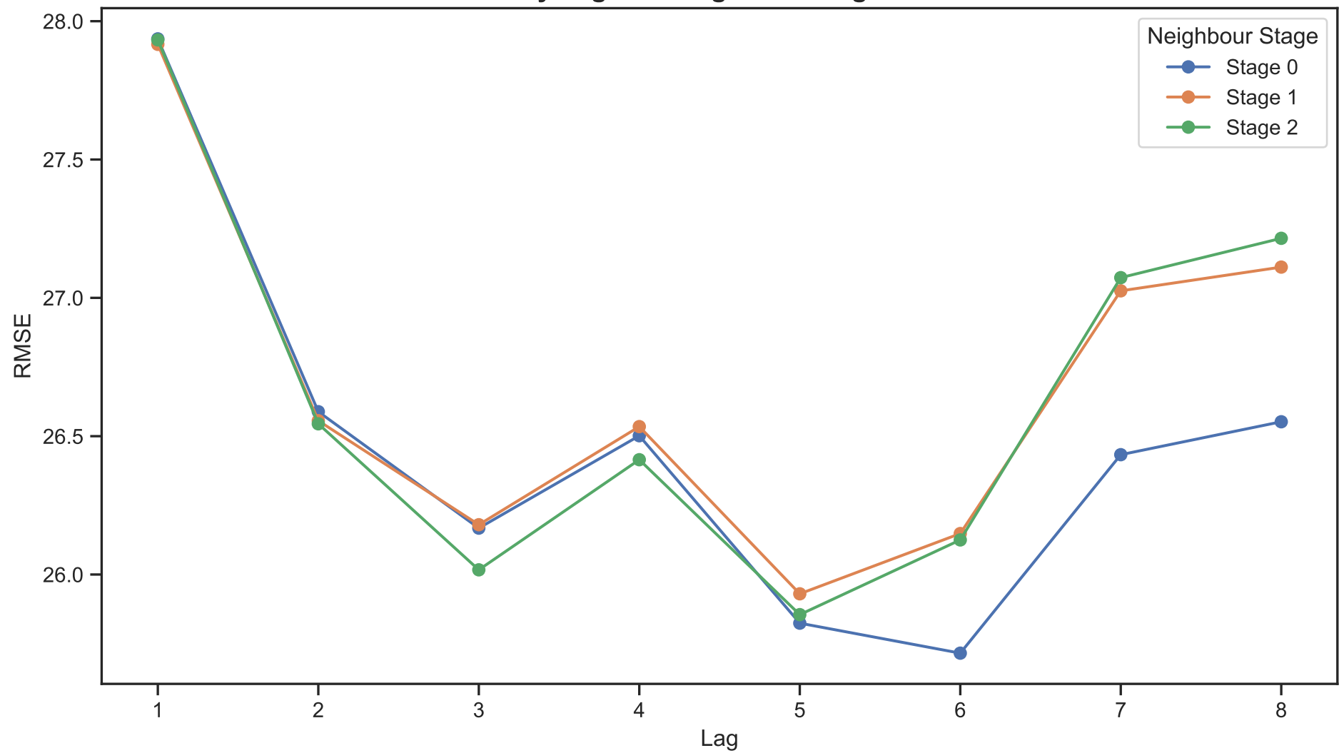
Mean RMSE by Lag and Neighbour Stage: No Covariates
