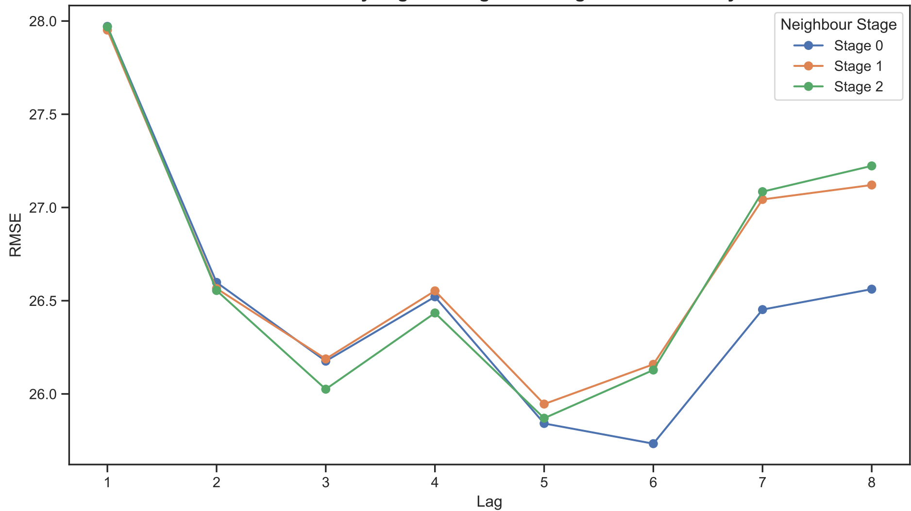
Mean RMSE by Lag and Neighbour Stage: Same Sex Only
