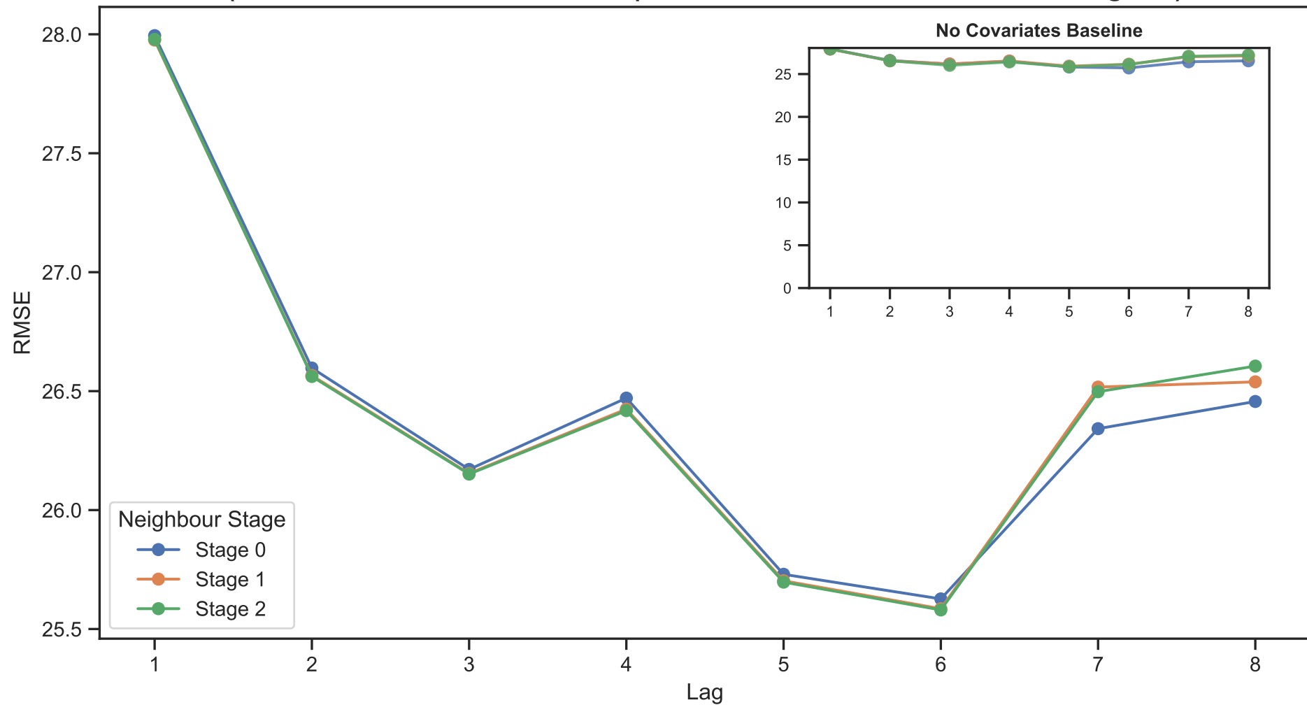
Mean RMSE by Lag and Neighbour Stage: Full Model (Main: Full Model Zoomed Detail | Inset: No-Covariates Baseline Starting at 0)
