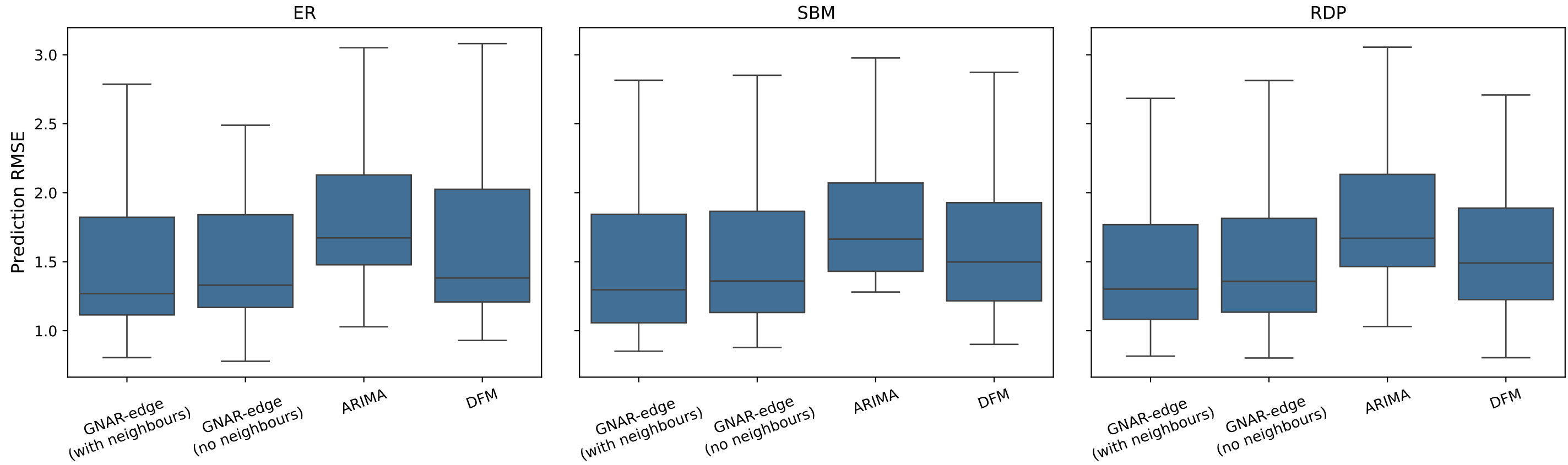
Prediction RMSE for Simulated Network on 13 Nodes, Density 0.436
