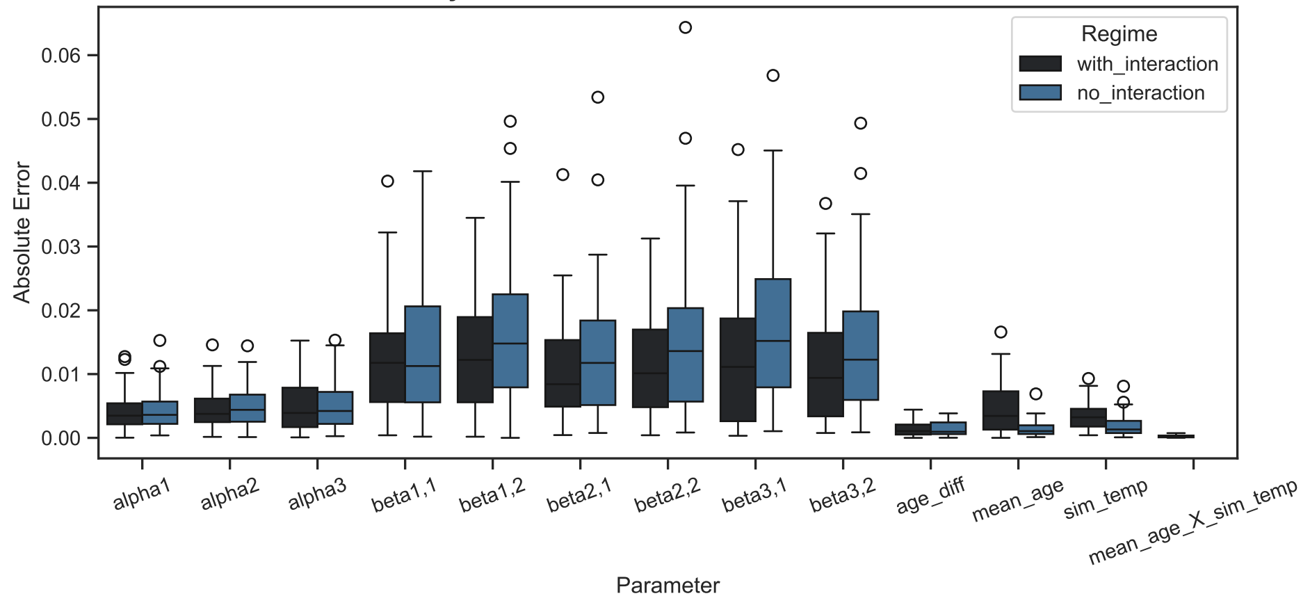
Absolute Error by Parameter, With vs. Without Interaction Term: RDP
