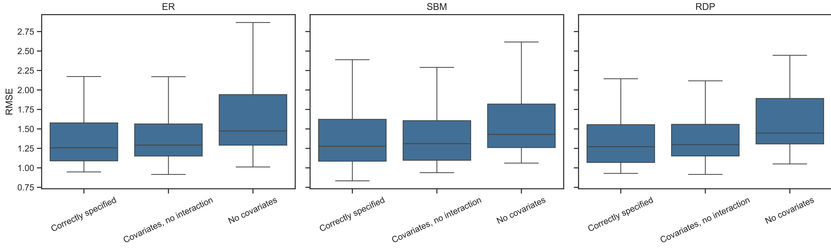
Prediction RMSE by fitted model, density = 0.4
