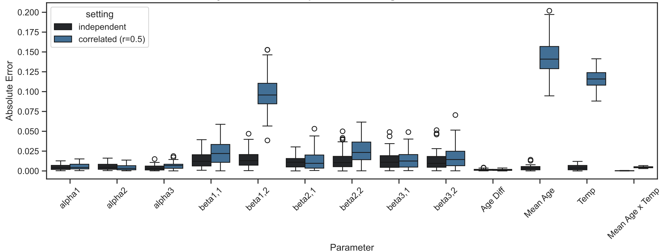
Absolute Error by Parameter, Independent vs Exogenous-Correlated Innovations: ER
