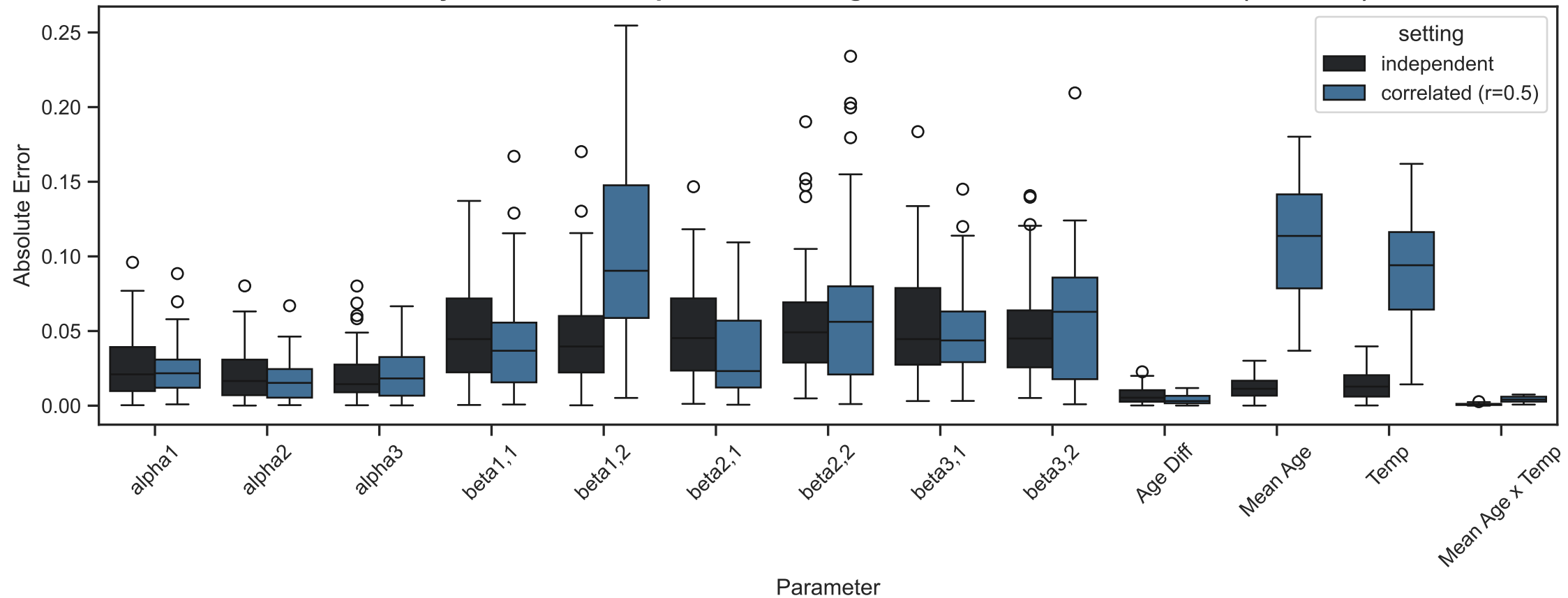
Absolute Error by Parameter, Independent vs Exogenous-Correlated Innovations (13 nodes): ER
