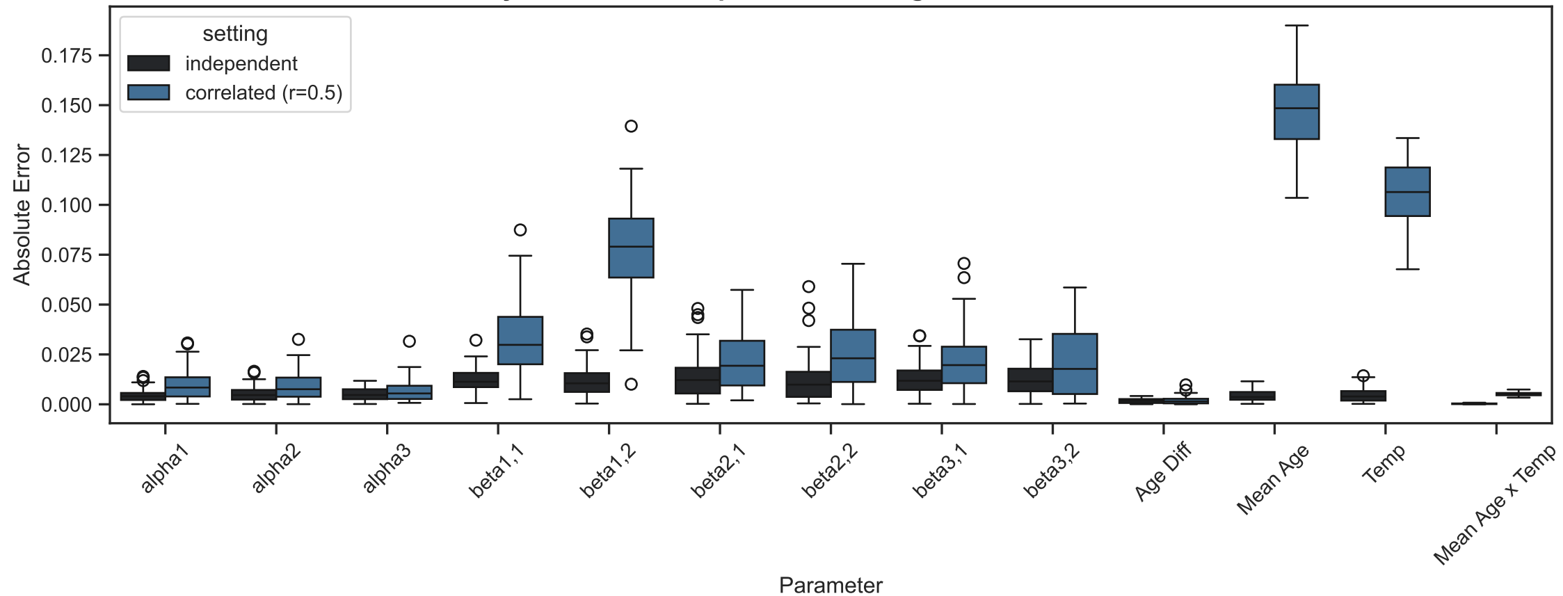
Absolute Error by Parameter, Independent vs Exogenous-Correlated Innovations: RDP
