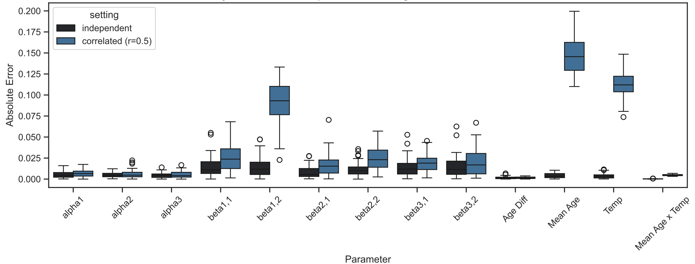
Absolute Error by Parameter, Independent vs Exogenous-Correlated Innovations: SBM
