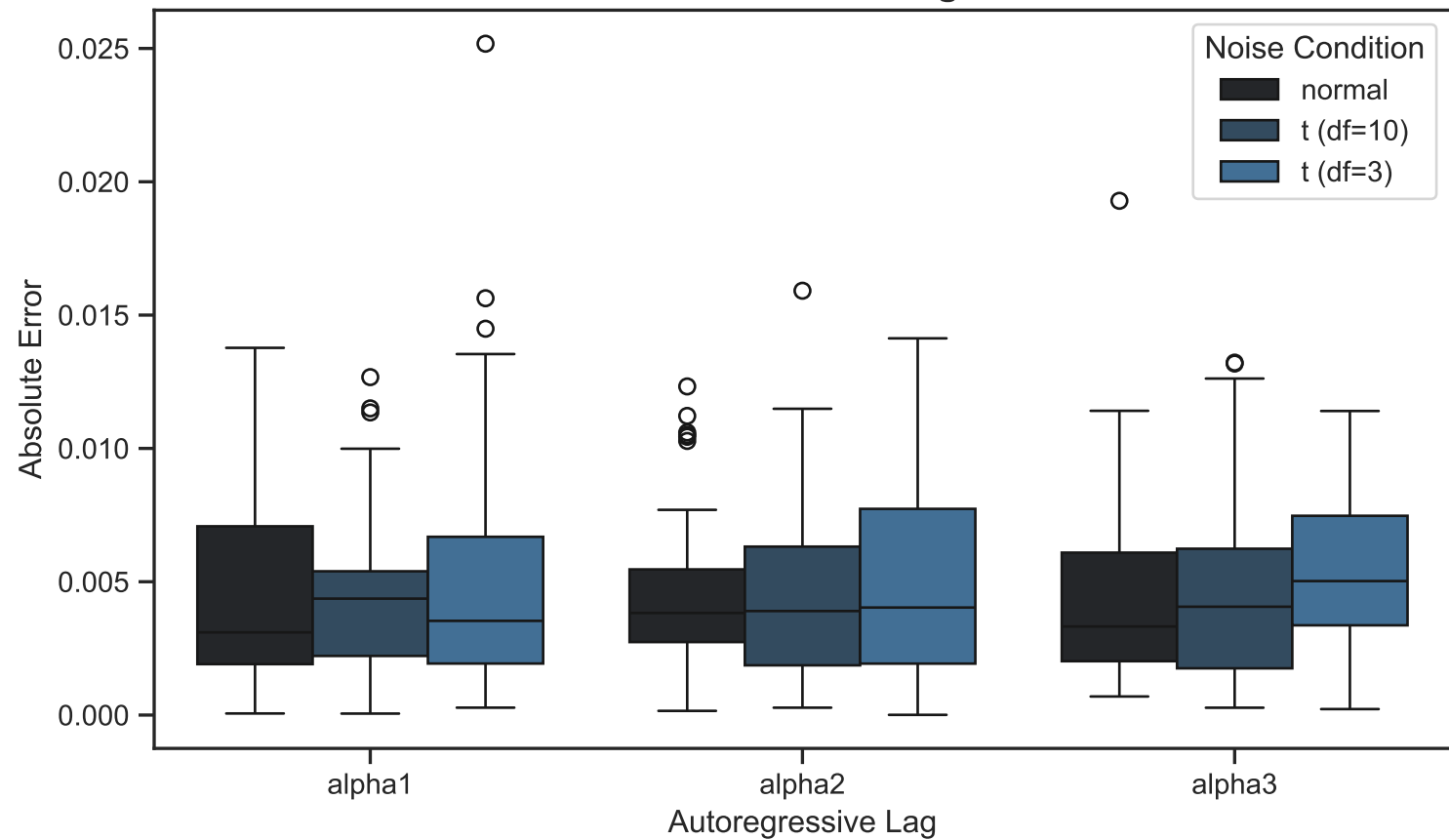
Distribution of Absolute Error for Autoregressive Parameters: ER
