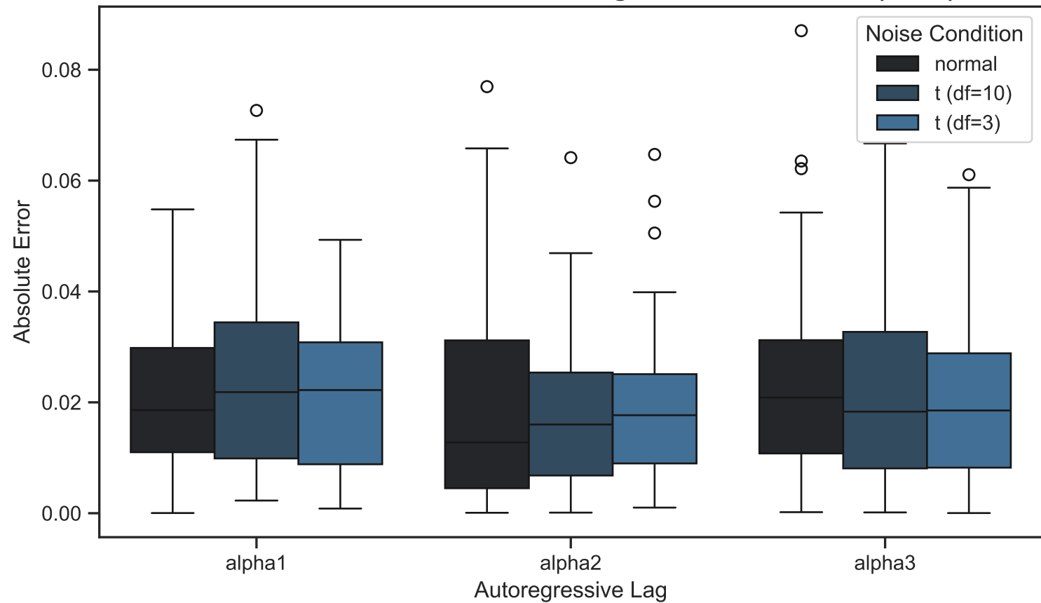
Distribution of Absolute Error for Autoregressive Parameters (K=13): SBM
