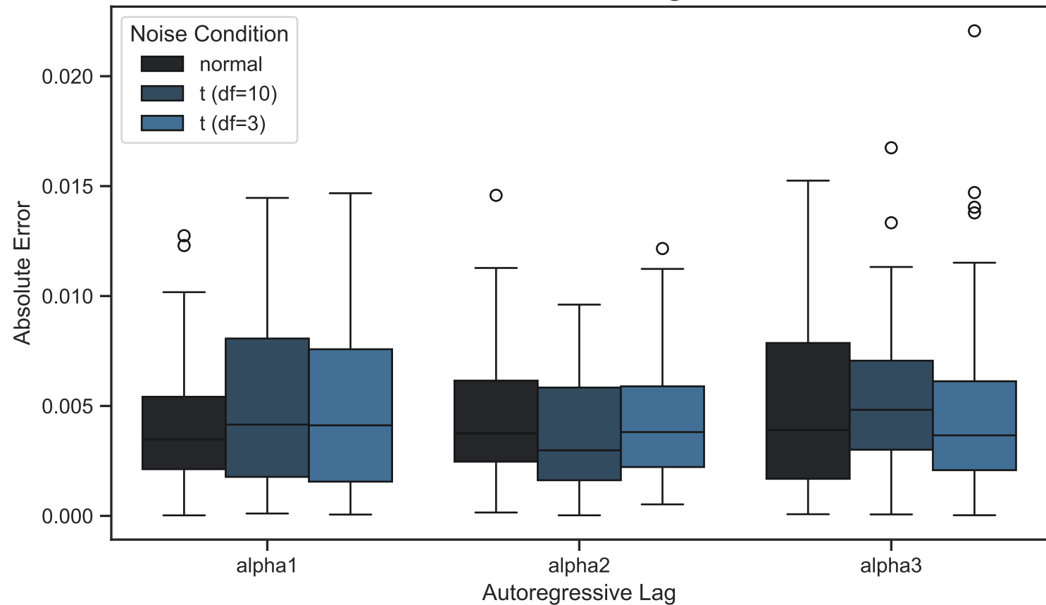
Distribution of Absolute Error for Autoregressive Parameters: RDP
