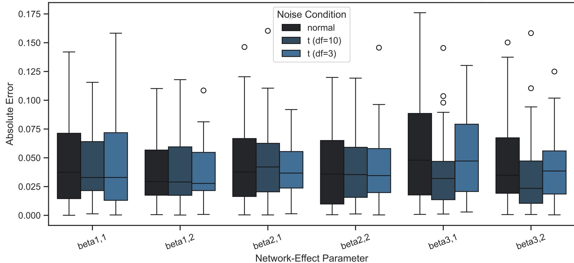
Distribution of Absolute Error for Network-Effect Parameters (K=13): ER
