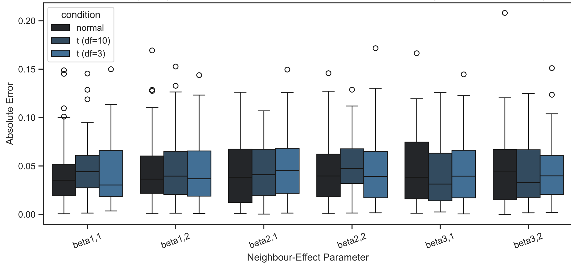
Absolute Error by Neighbour-Effect Parameter, Innovation Distribution (No Interaction Term): ER
