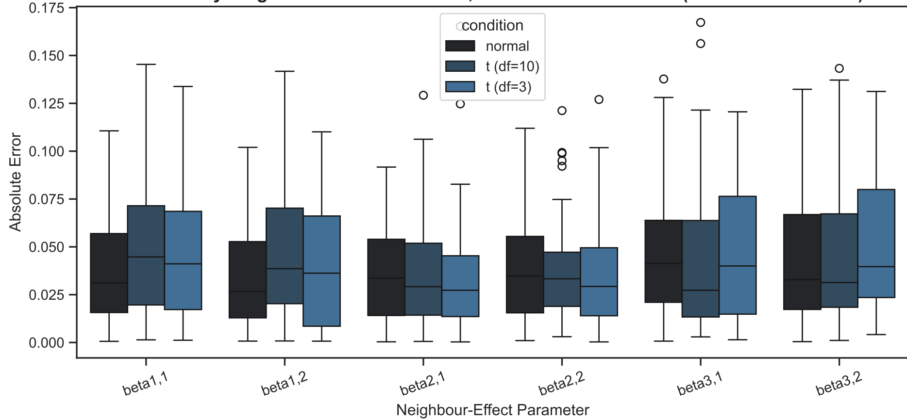
Absolute Error by Neighbour-Effect Parameter, Innovation Distribution (No Interaction Term): SBM
