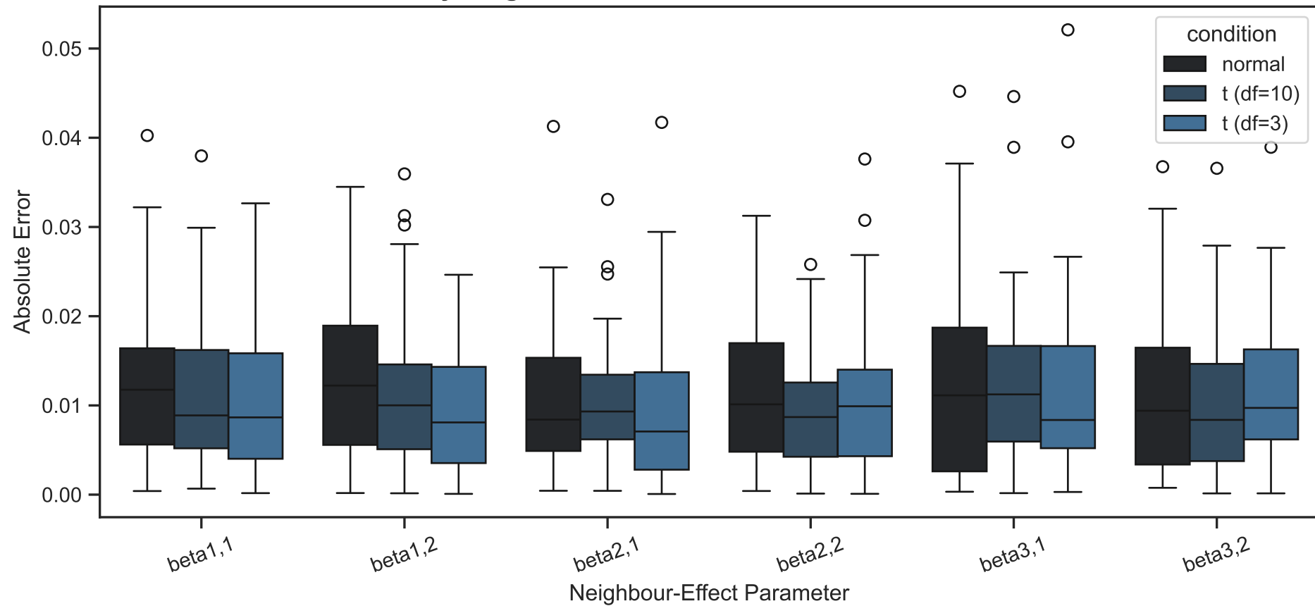
Absolute Error by Neighbour-Effect Parameter, Innovation Distribution: RDP
