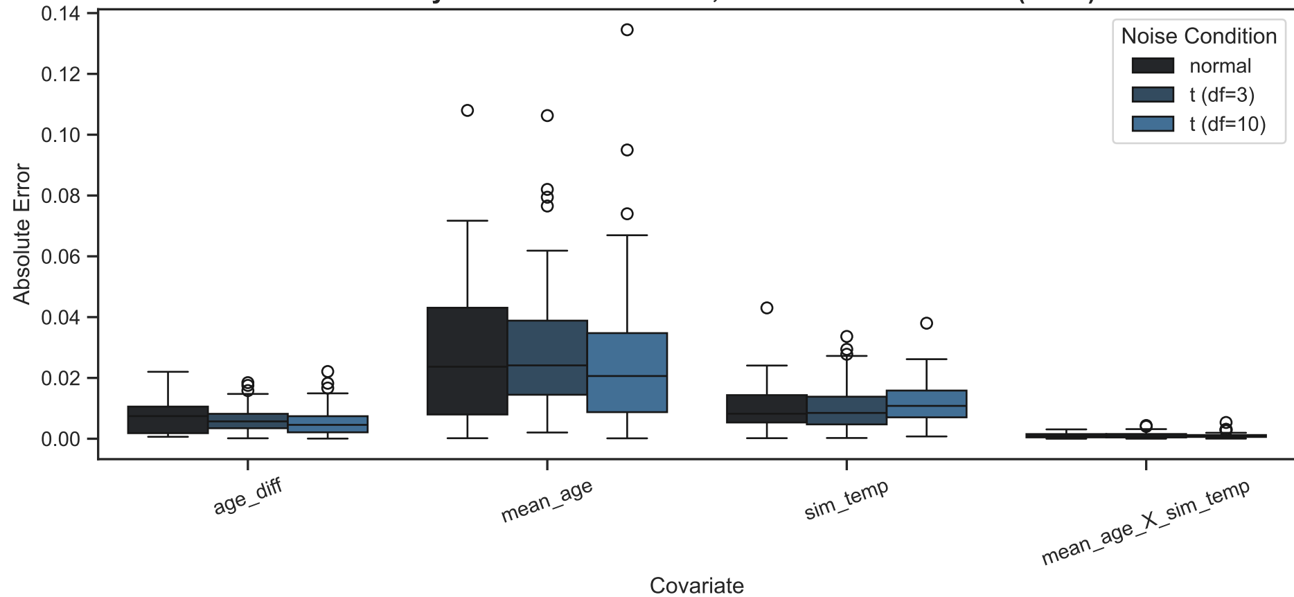
Absolute Error by Covariate Coefficient, Innovation Distribution (K=13): RDP
