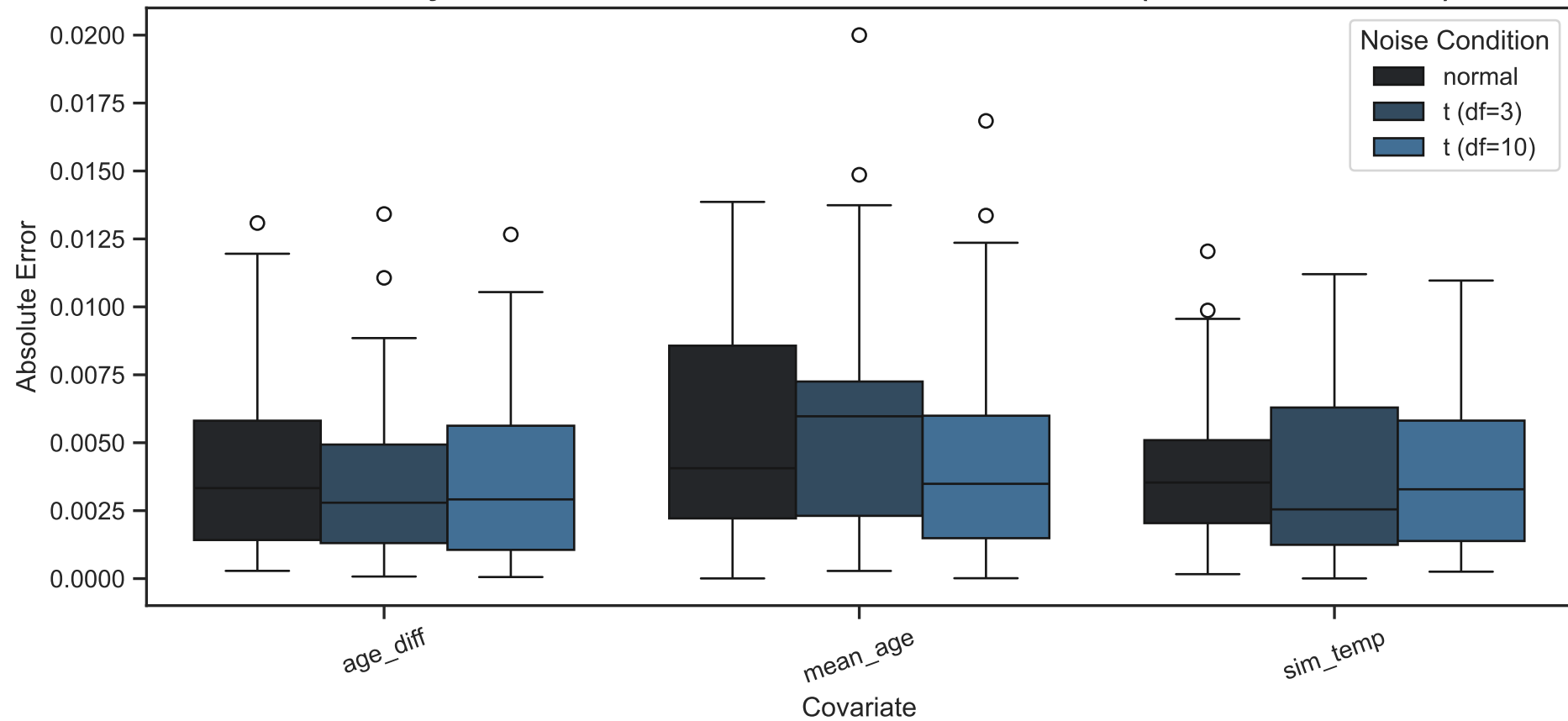
Absolute Error by Covariate Coefficient, Innovation Distribution (No Interaction Term): RDP
