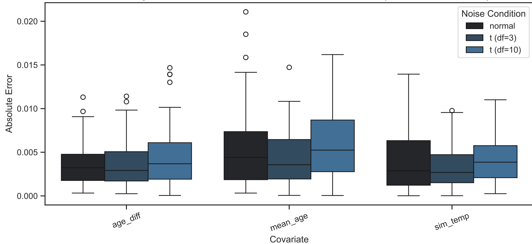
Absolute Error by Covariate Coefficient, Innovation Distribution (No Interaction Term): SBM
