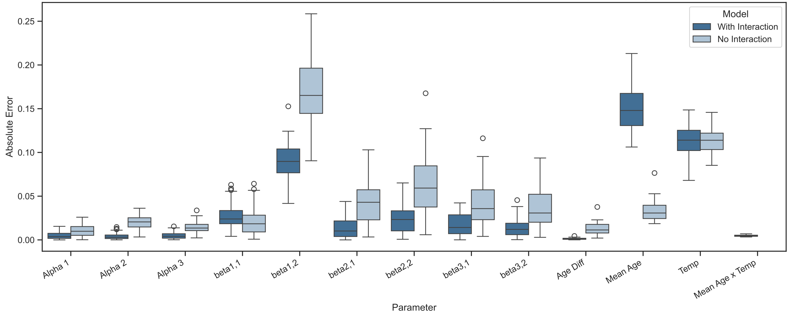
Absolute Error by Parameter, With vs Without Interaction Term (Exogenous Correlation = 0.5): ER
