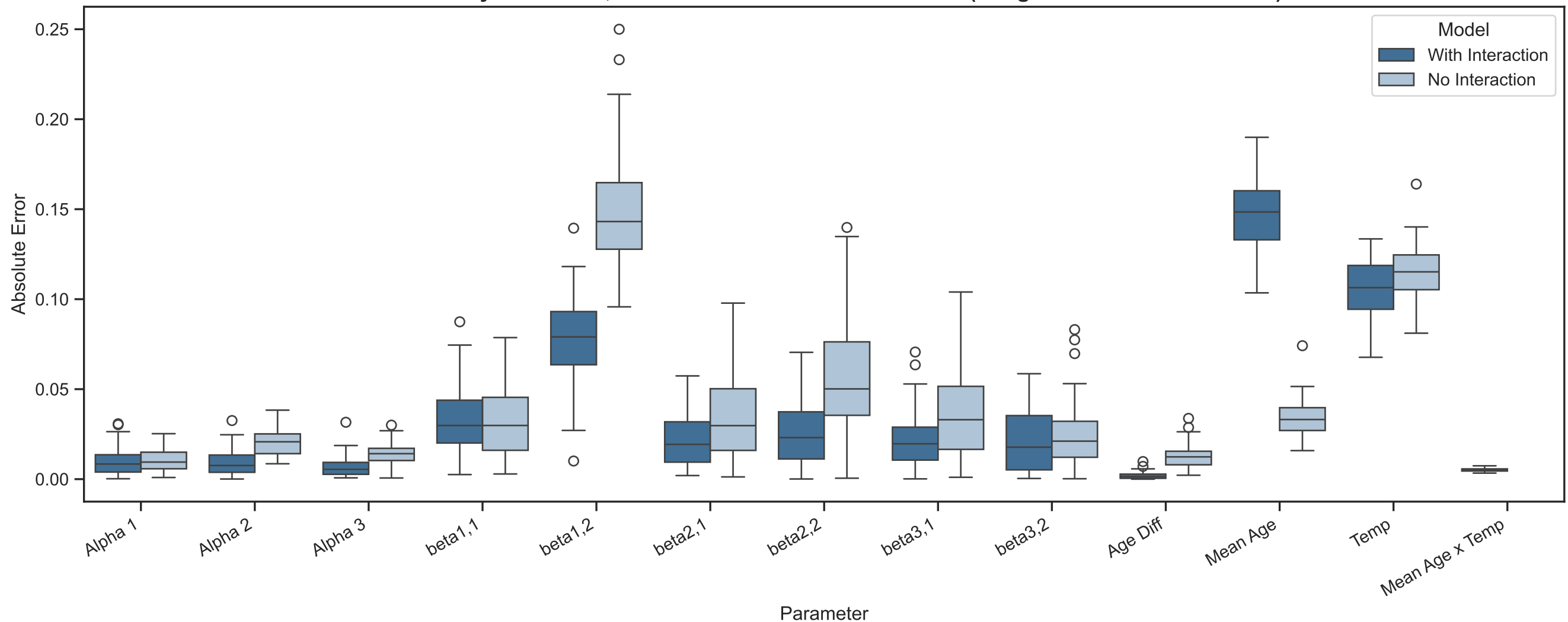
Absolute Error by Parameter, With vs Without Interaction Term (Exogenous Correlation = 0.5): RDP
