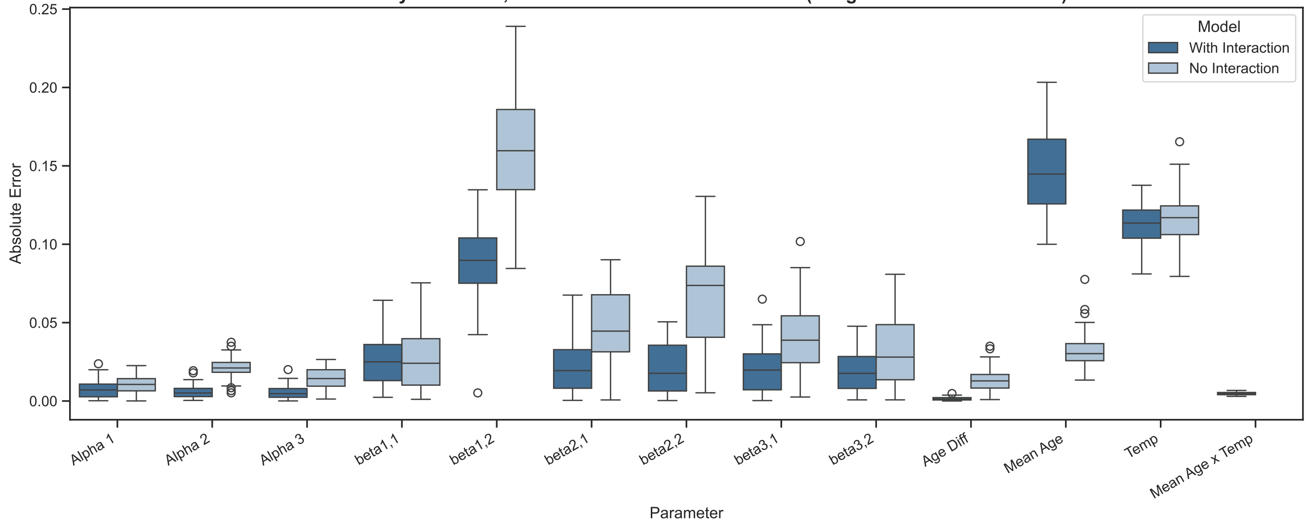
Absolute Error by Parameter, With vs Without Interaction Term (Exogenous Correlation = 0.5): SBM
