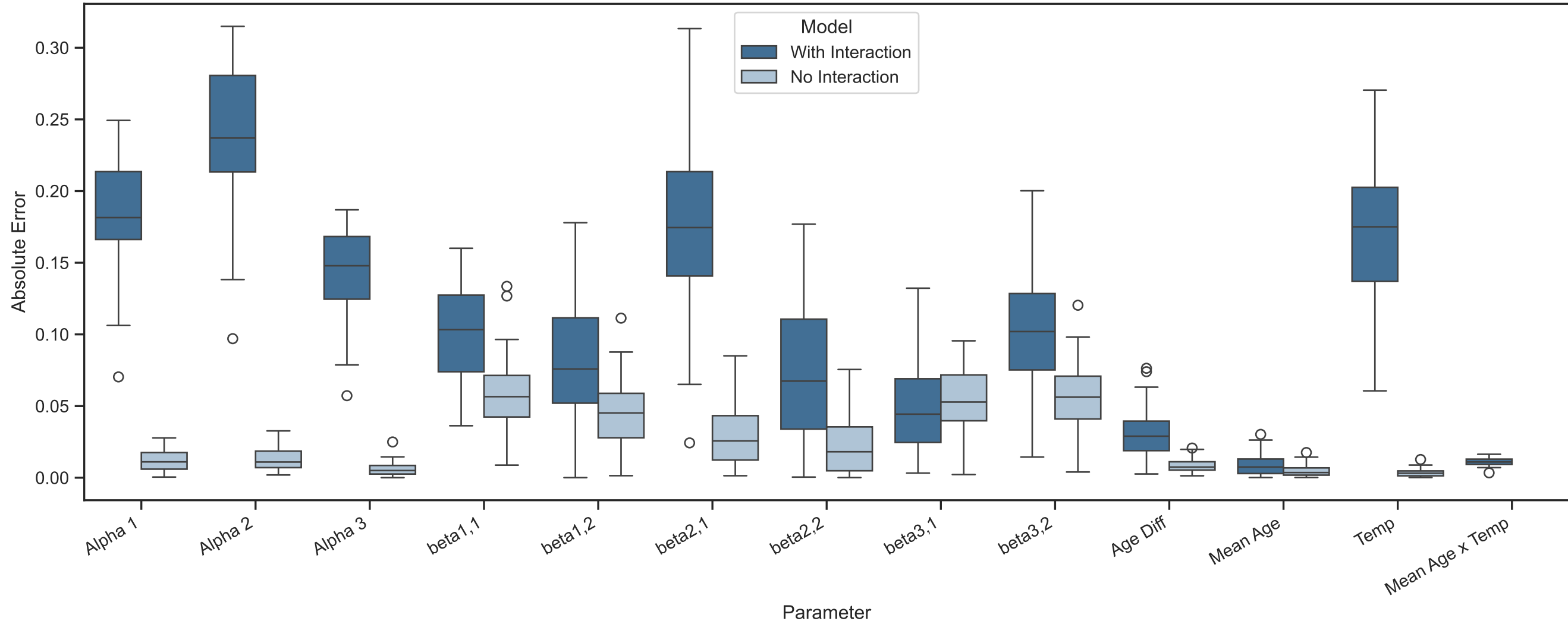
Absolute Error by Parameter, With vs Without Interaction Term (Rewiring Probability = 0.2): ER
