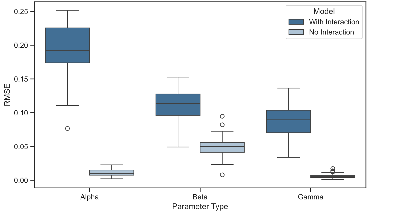
RMSE by Parameter Type, With vs Without Interaction Term (Rewiring Probability = 0.2): ER
