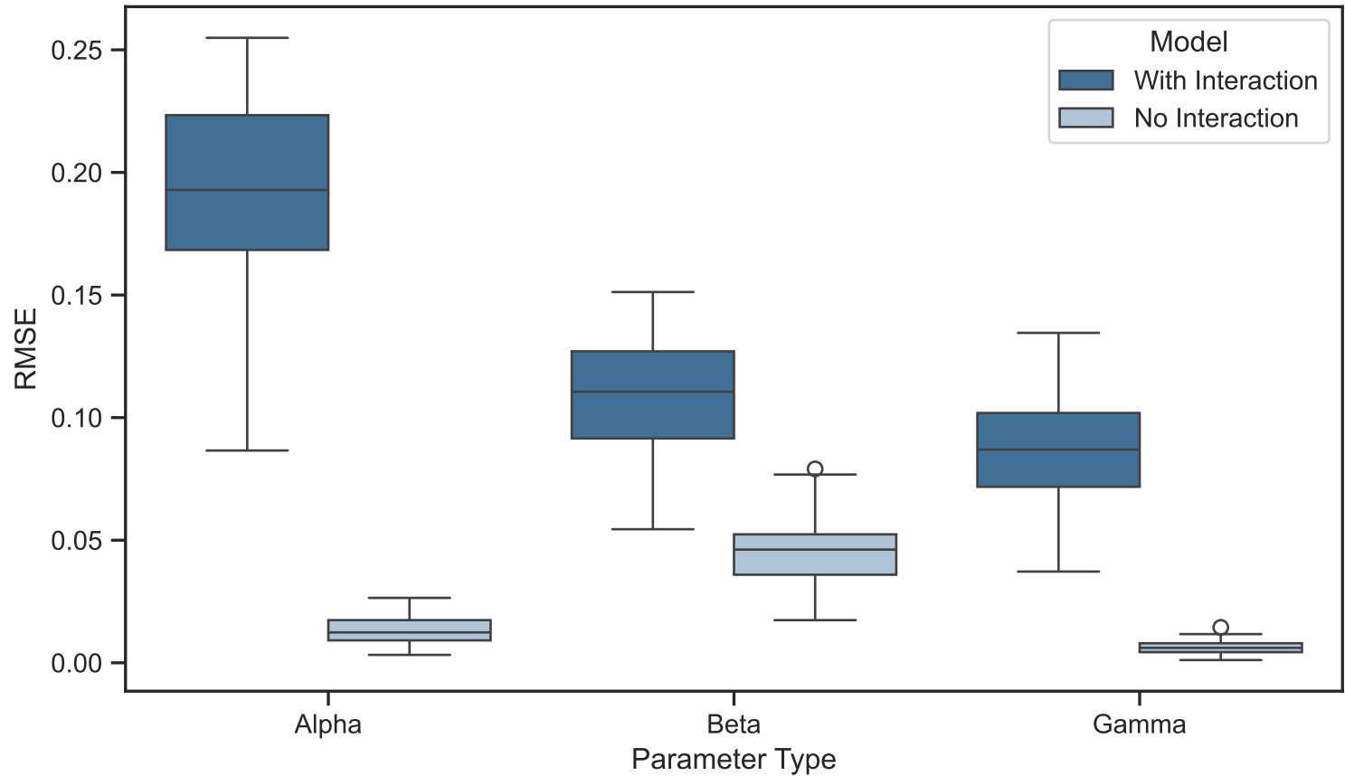
RMSE by Parameter Type, With vs Without Interaction Term (Rewiring Probability = 0.2): SBM
