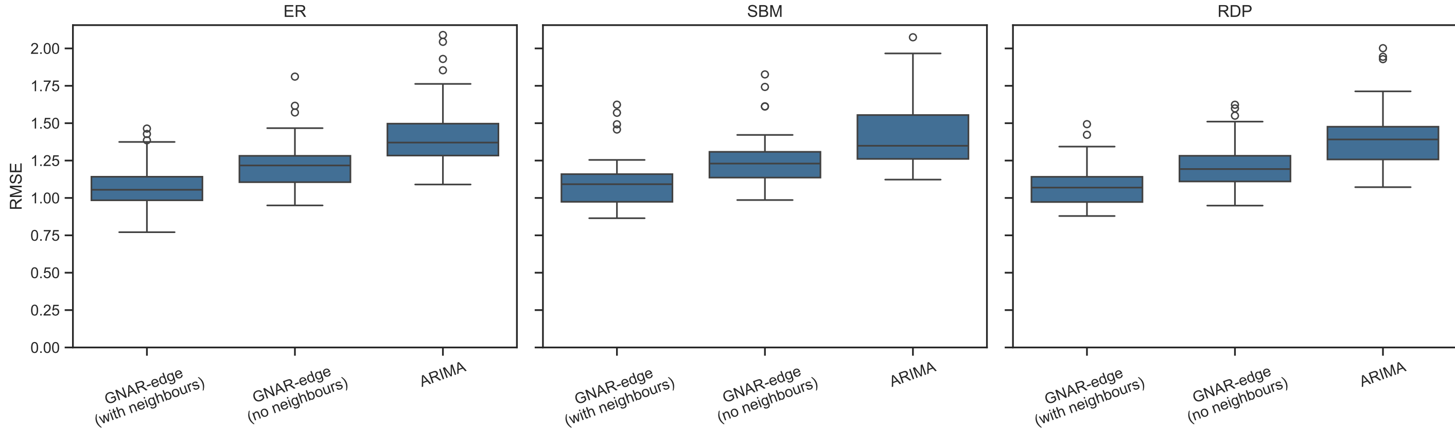
with_covariates_no_interaction (regime 8), density = 0.4
