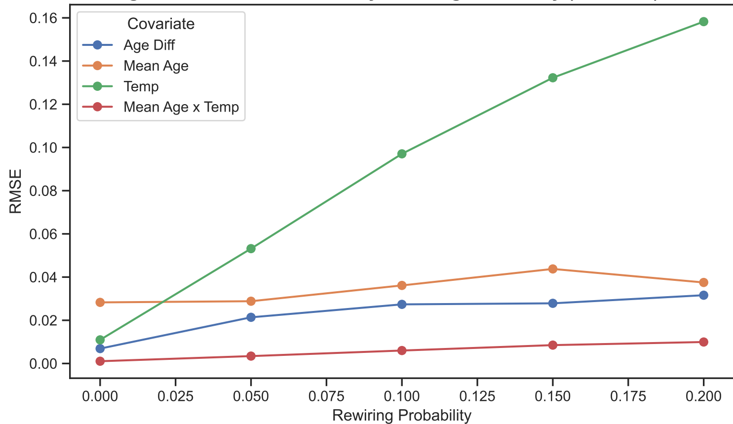
Exogenous Coefficient RMSE by Rewiring Probability (13 nodes): RDP
