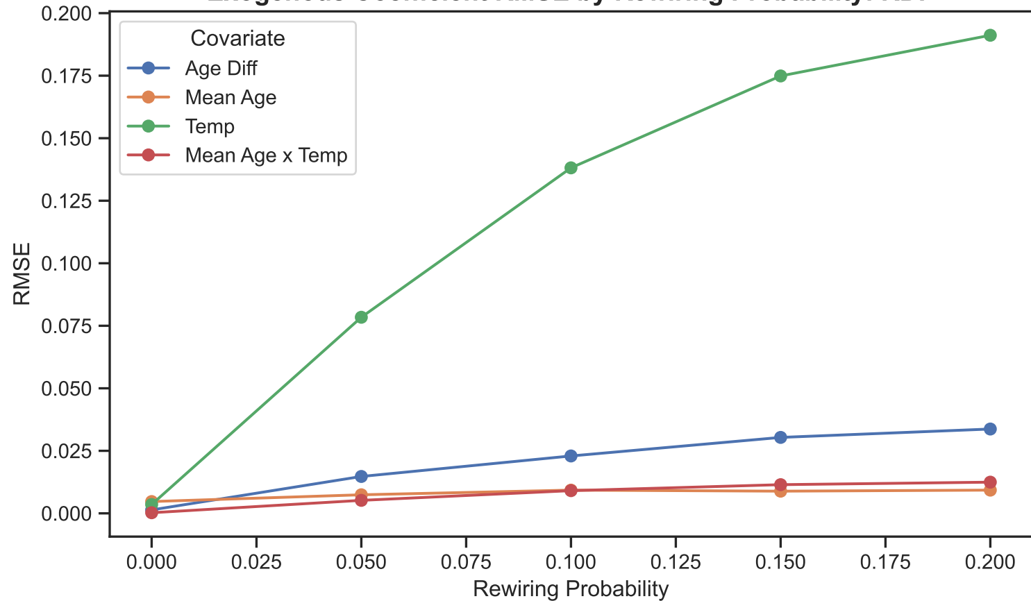
Exogenous Coefficient RMSE by Rewiring Probability: RDP
