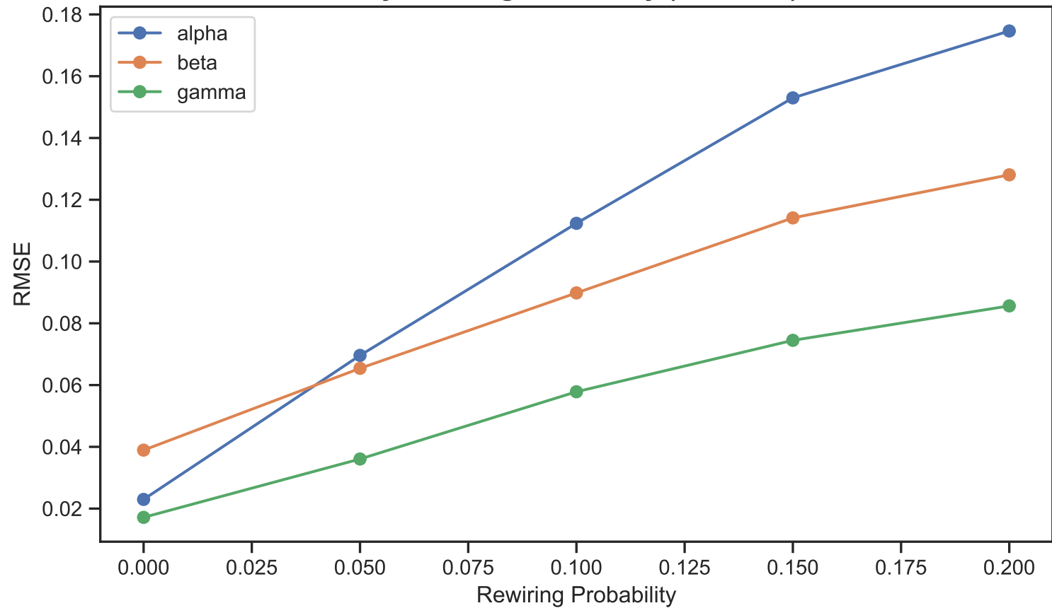
RMSE by Rewiring Probability (13 nodes): RDP
