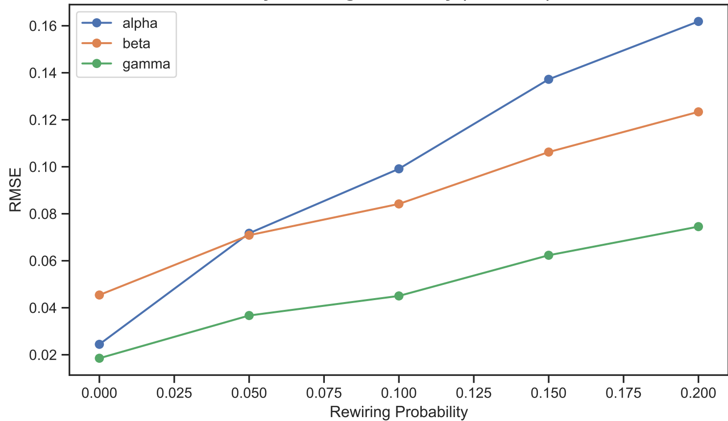
RMSE by Rewiring Probability (13 nodes): SBM
