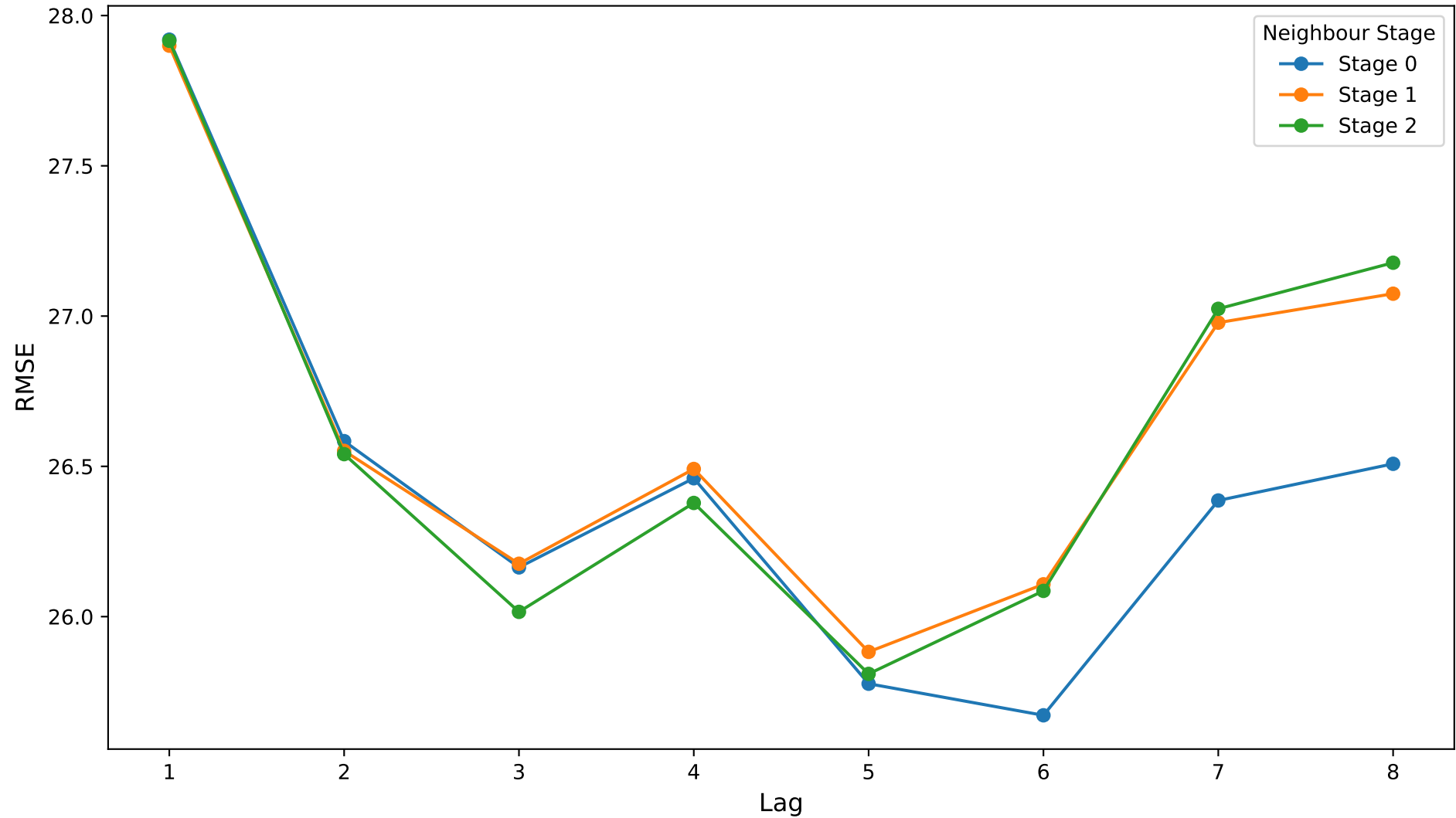
Mean RMSE by Lag and Neighbour Stage: Age Difference, Mean Age
