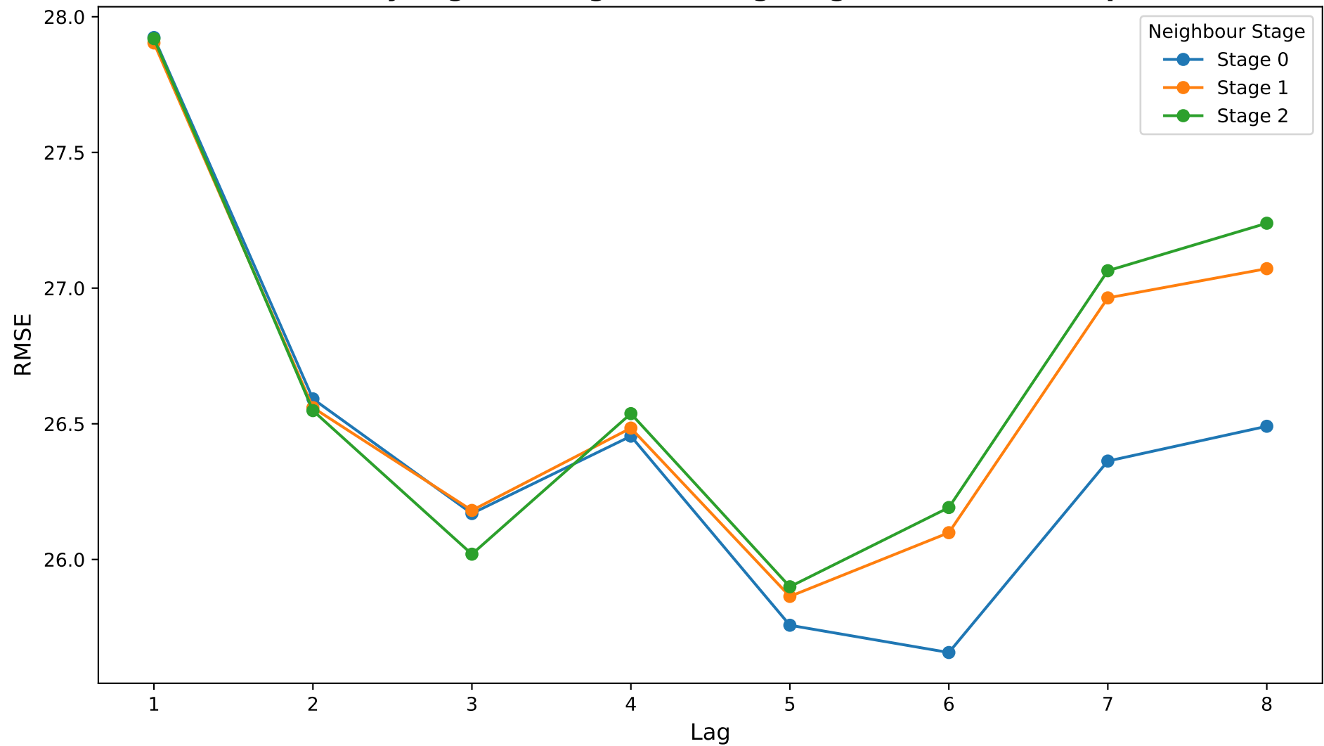
Mean RMSE by Lag and Neighbour Stage: Age Difference, Temperature
