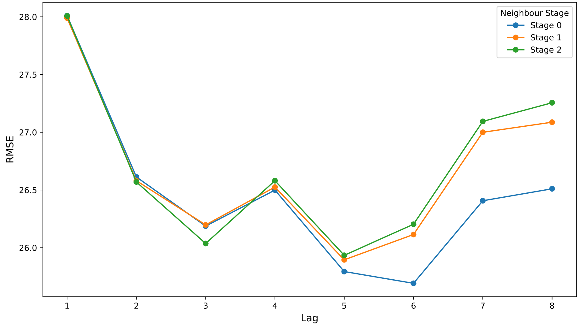
Mean RMSE by Lag and Neighbour Stage: age_diff_temp_same_sex
