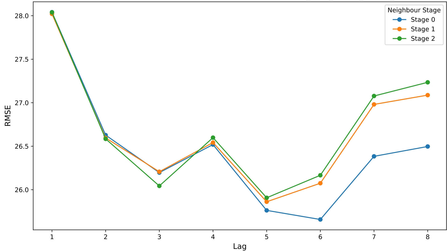
Mean RMSE by Lag and Neighbour Stage: mean_age_temp_same_sex
