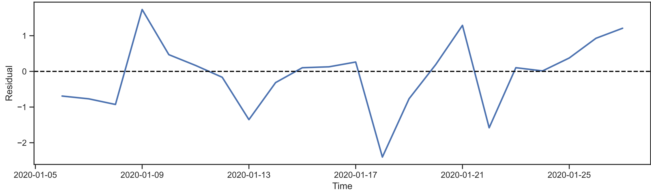
T = 28: residuals (1->2)
