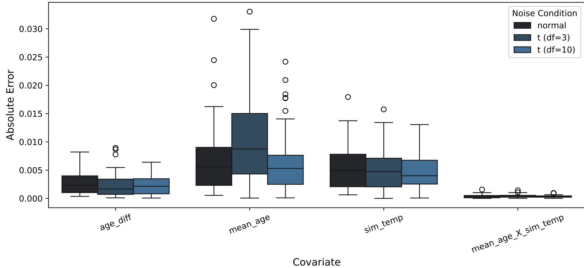
Absolute Error by Covariate Coefficient, Innovation Distribution (K=13): ER
