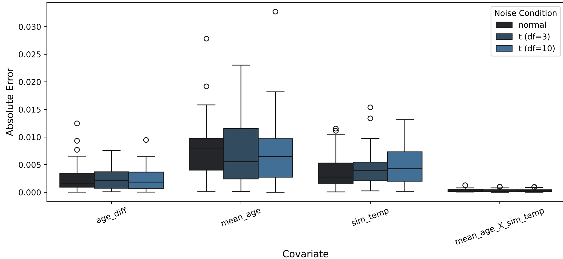
Absolute Error by Covariate Coefficient, Innovation Distribution (K=13): RDP
